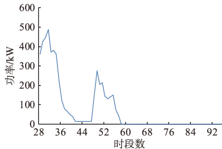
图 3 园区充电站的充电负荷 Fig.3 Charging load of the charging station in the park
