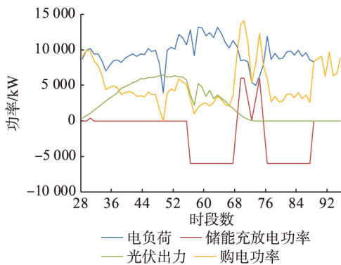
图 5 储能功率和购电功率 Fig.5 Energy storage power and purchasing power
