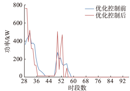
图 4 优化控制前后充电负荷对比 Fig.4 Comparison of charging load before and after optimized control
